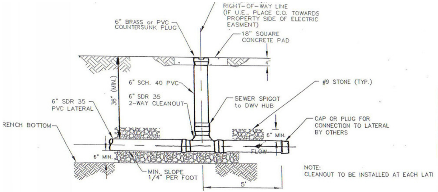
CLEANOUT DETAIL NTS
