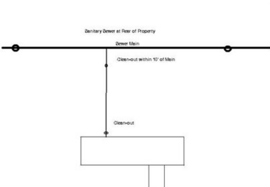
CLEANOUT DETAIL NTS
